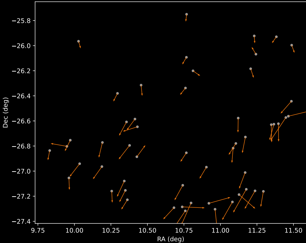
APOGEE DR17 Cluster 2 Proper Motion Vectors (n=53)
