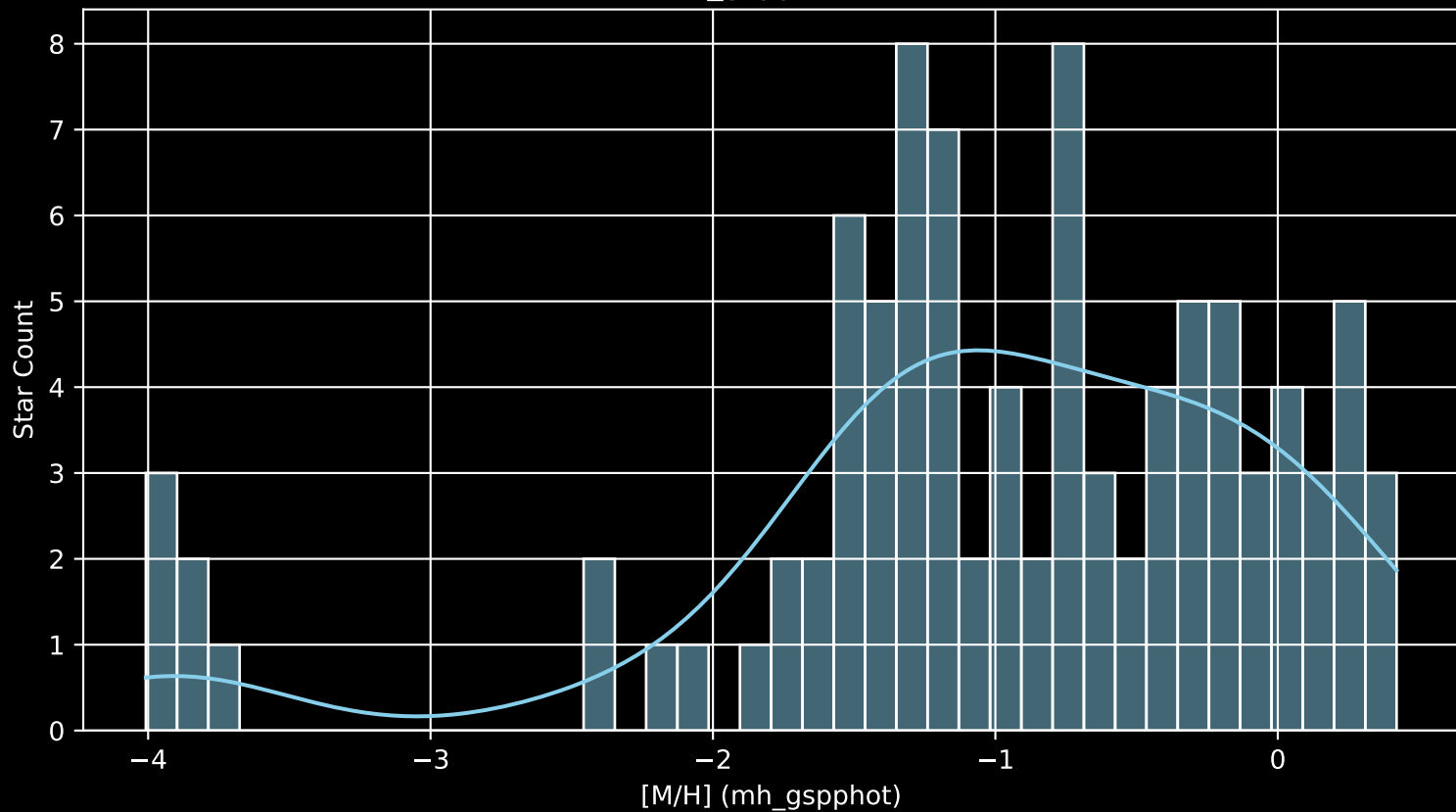
APOGEE DR17 Field: [004-02-O [M/H] (mh_gspphot) (n= 94)
