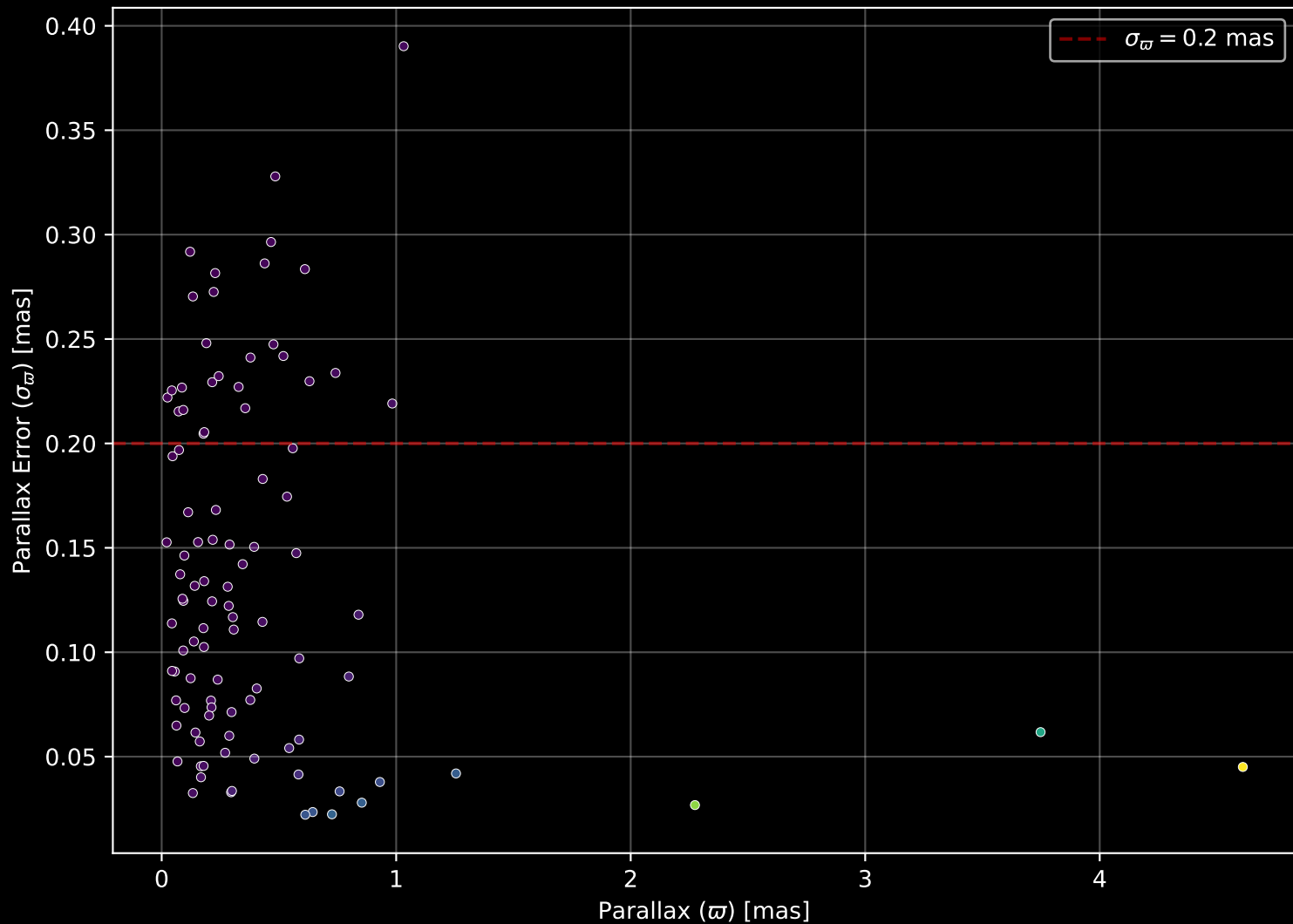
APOGEE DR17 Field: [004-02-O] Parallax Quality (n= 99)
