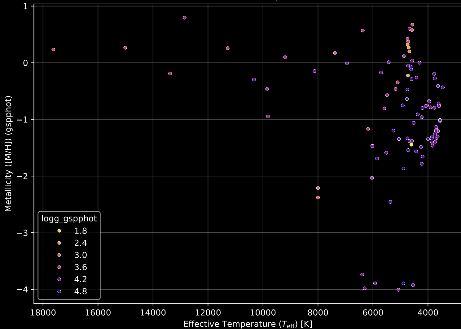
APOGEE DR17 Field: [004-02-O] Stellar Population Parameters (n= 99)
