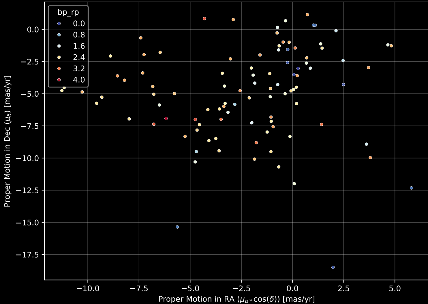
APOGEE DR17 Field: [004-02-O] Proper Motion Diagram (n= 99)
